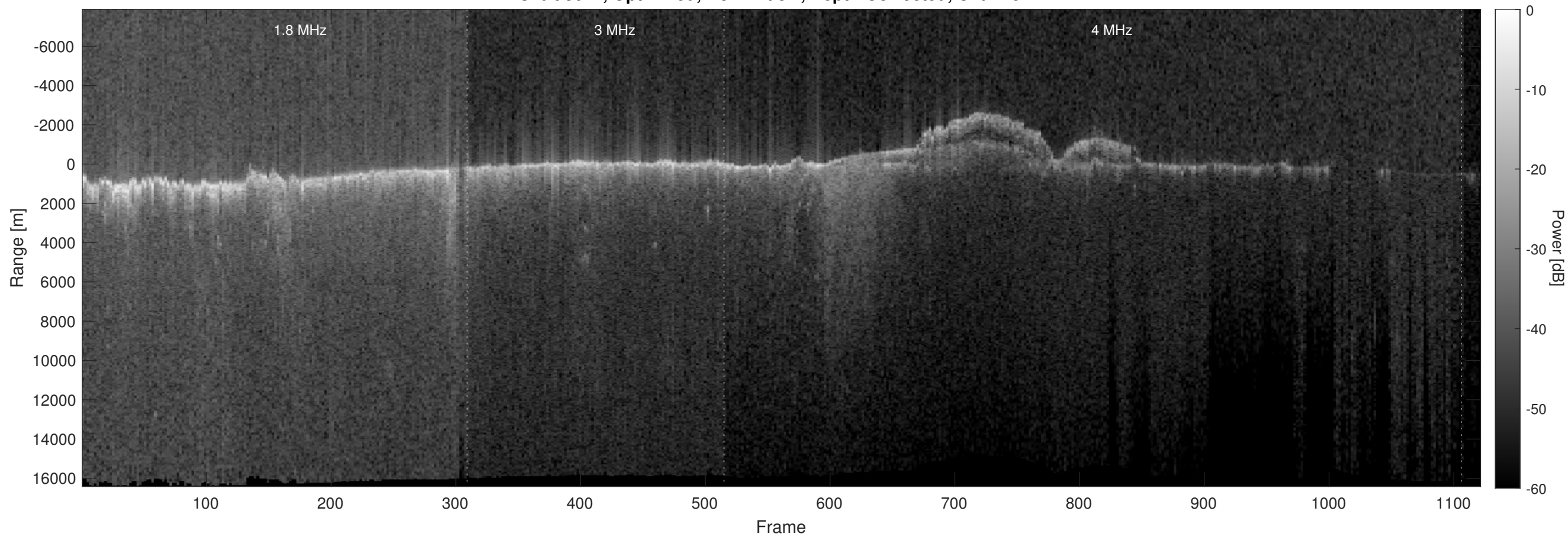
Orbit 3674, Optimized, No Window, Depth-Corrected, Channel 2
