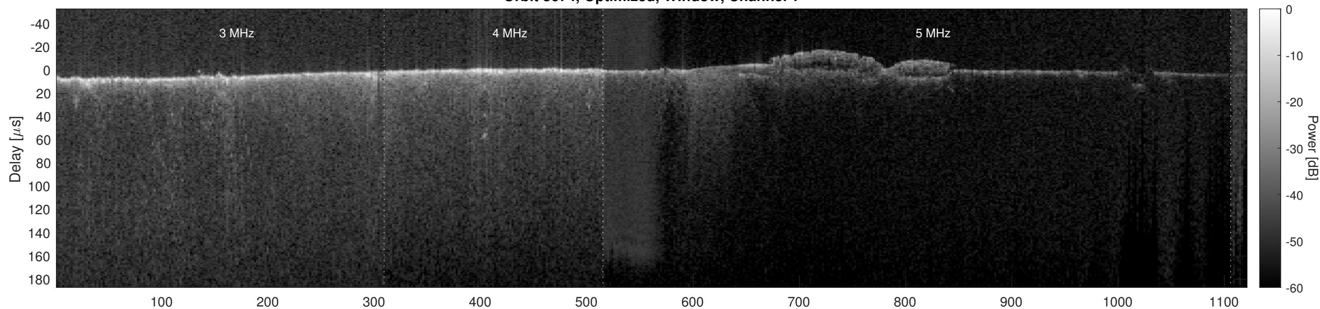
Orbit 3674, Optimized, Window, Channel 2
