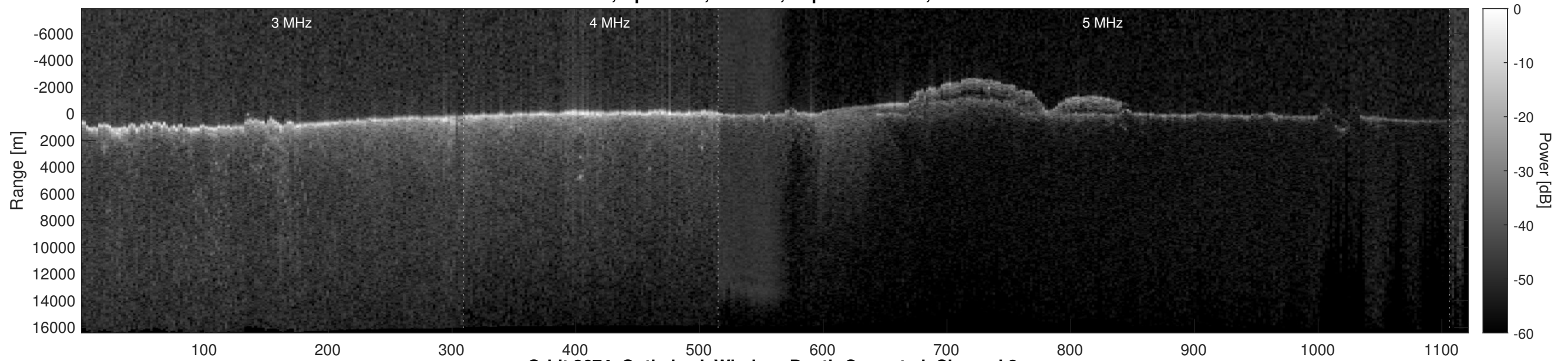
Orbit 3674, Optimized, Window, Depth-Corrected, Channel 2
