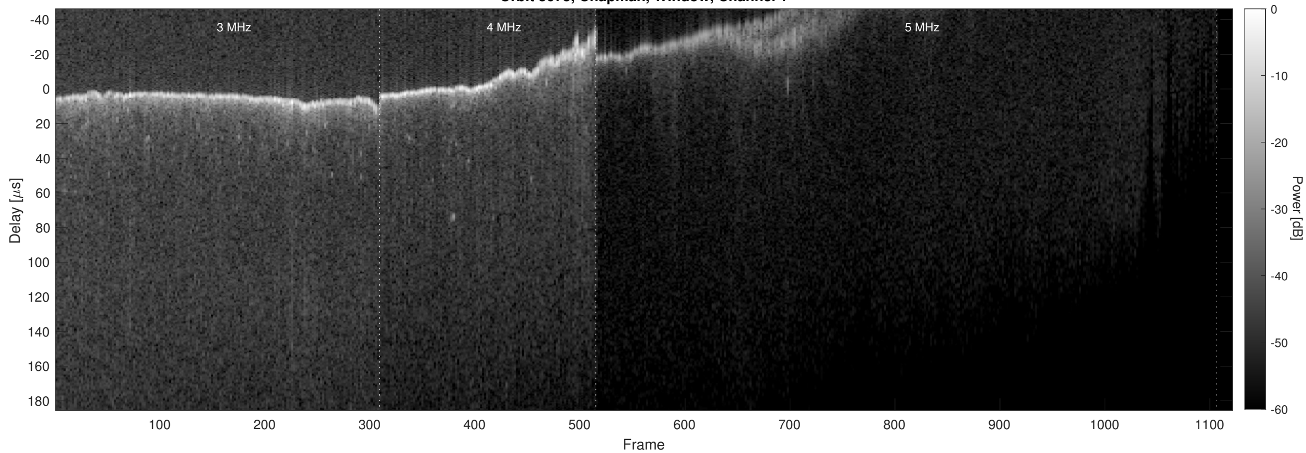
Orbit 3675, Chapman, Window, Channel 2
