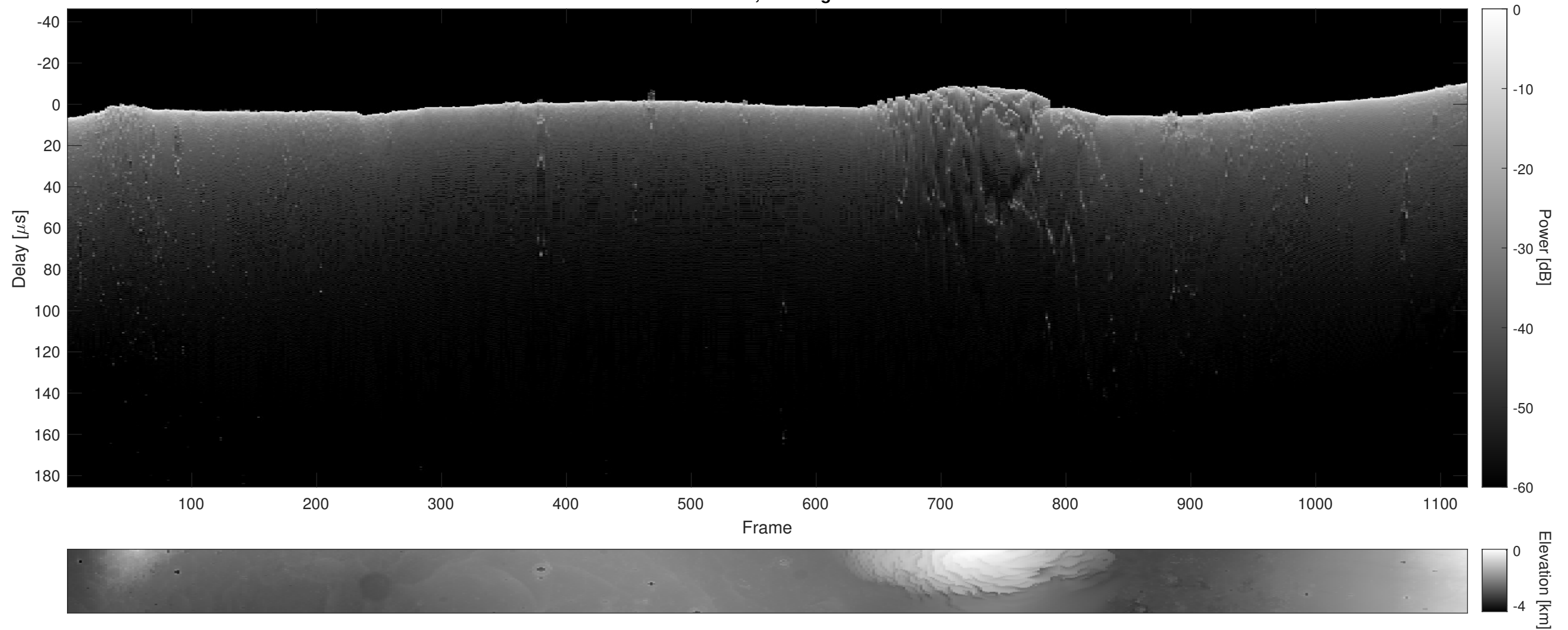
Orbit 3675, Cluttergram
