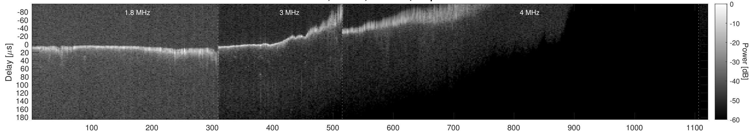
Orbit 3675, Window, Channel 2, Optimized
