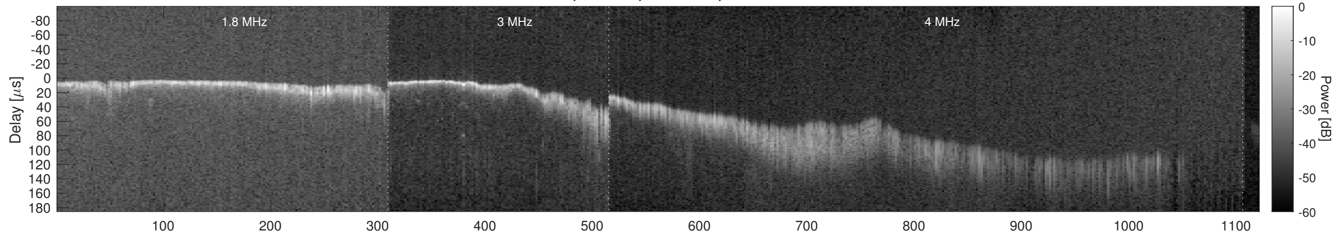
Orbit 3675, Window, Channel 2, Chapman
