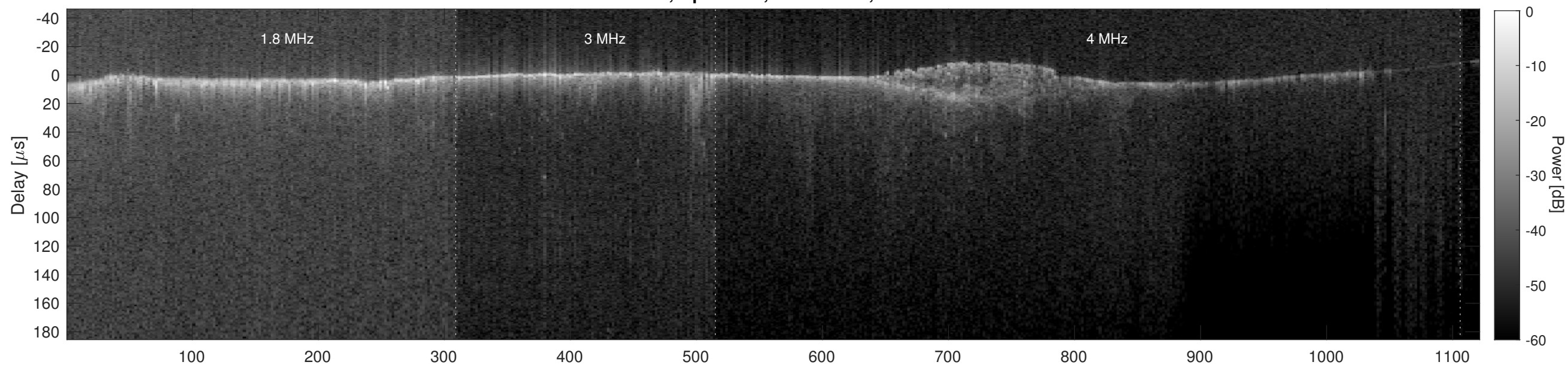
Orbit 3675, Cluttergram
