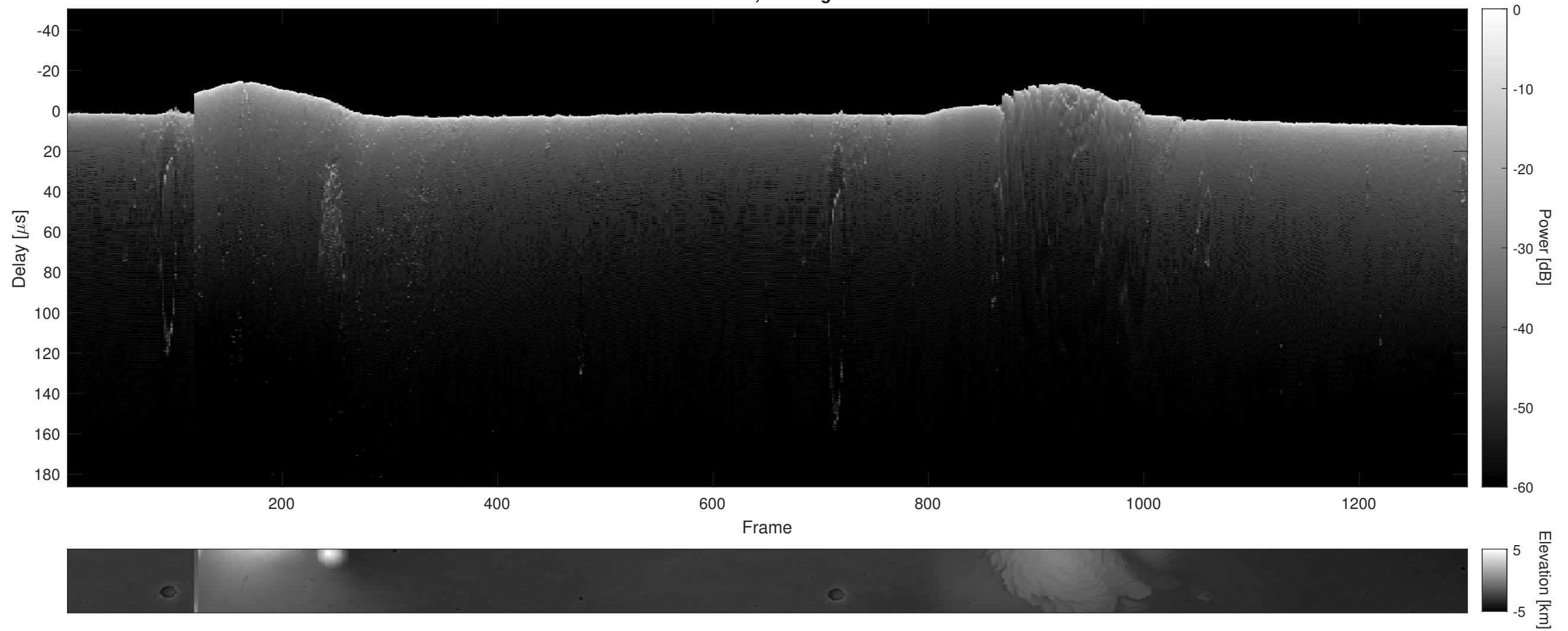
Orbit 3678, Cluttergram
