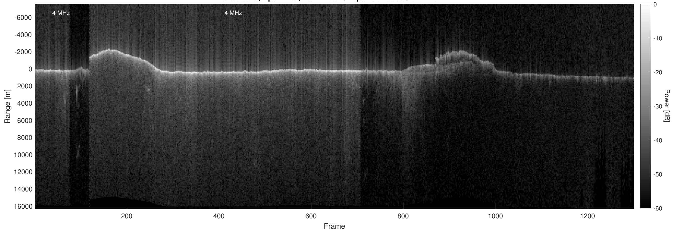
Orbit 3678, Optimized, No Window, Depth-Corrected, Channel 2
