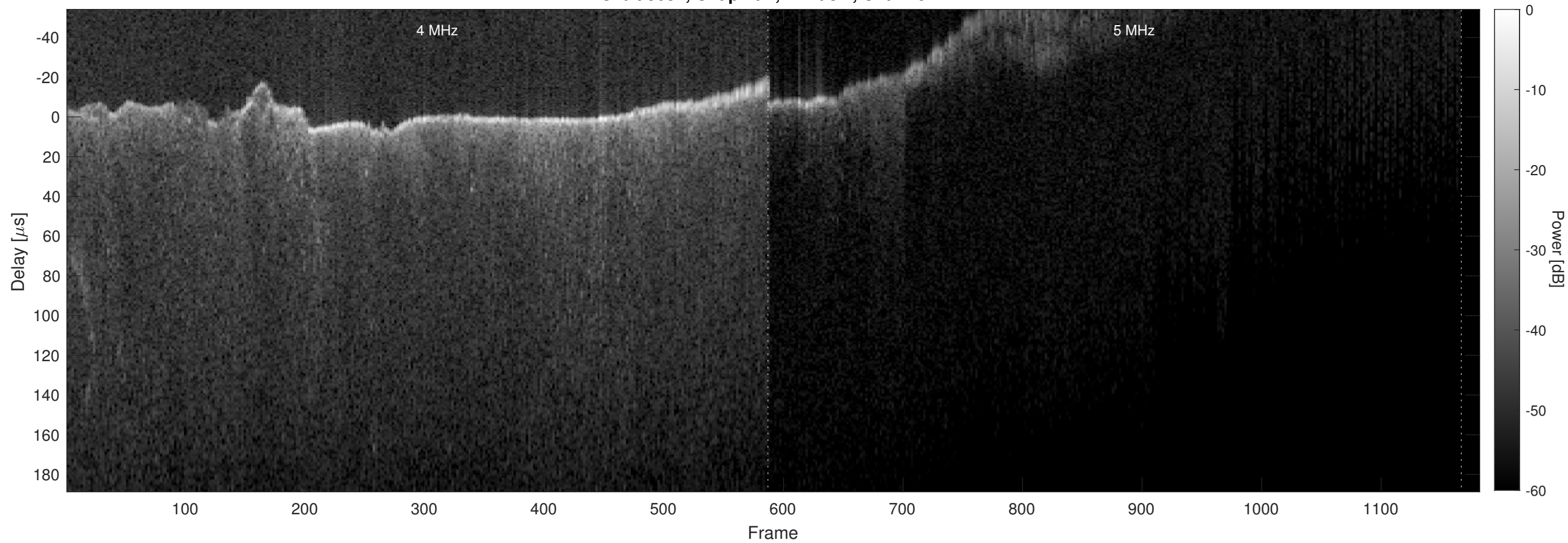
Orbit 3681, Chapman, Window, Channel 2
