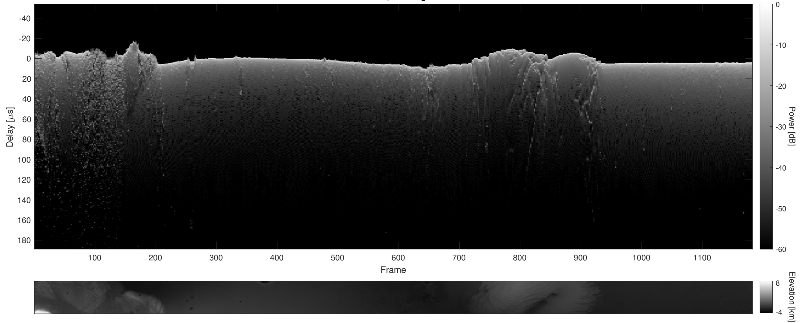
Orbit 3681, Cluttergram
