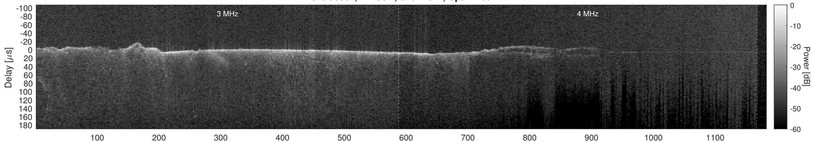
Orbit 3681, Cluttergram
