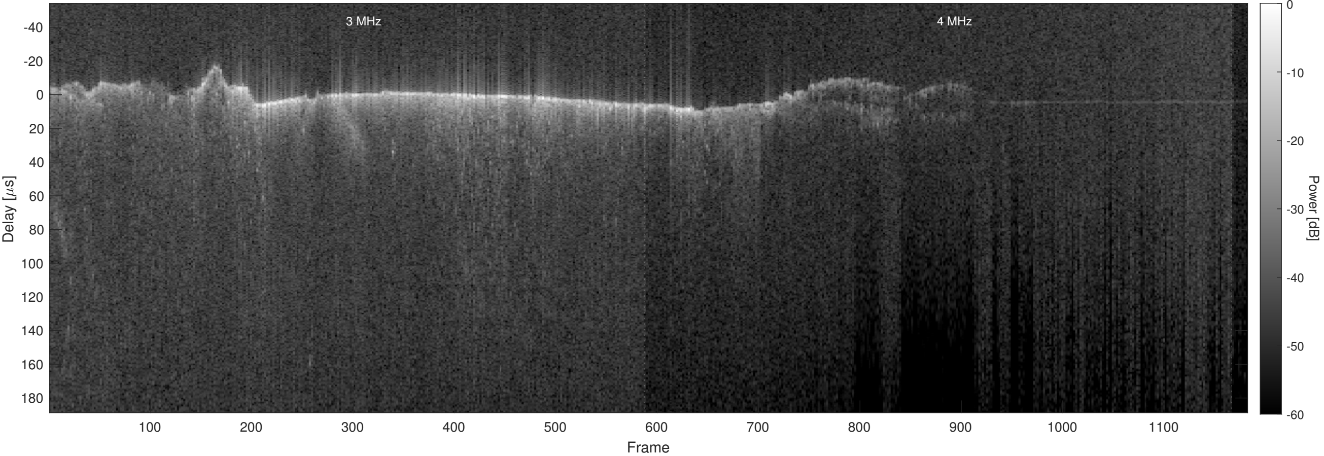
Orbit 3681, Optimized, No Window, Channel 2
