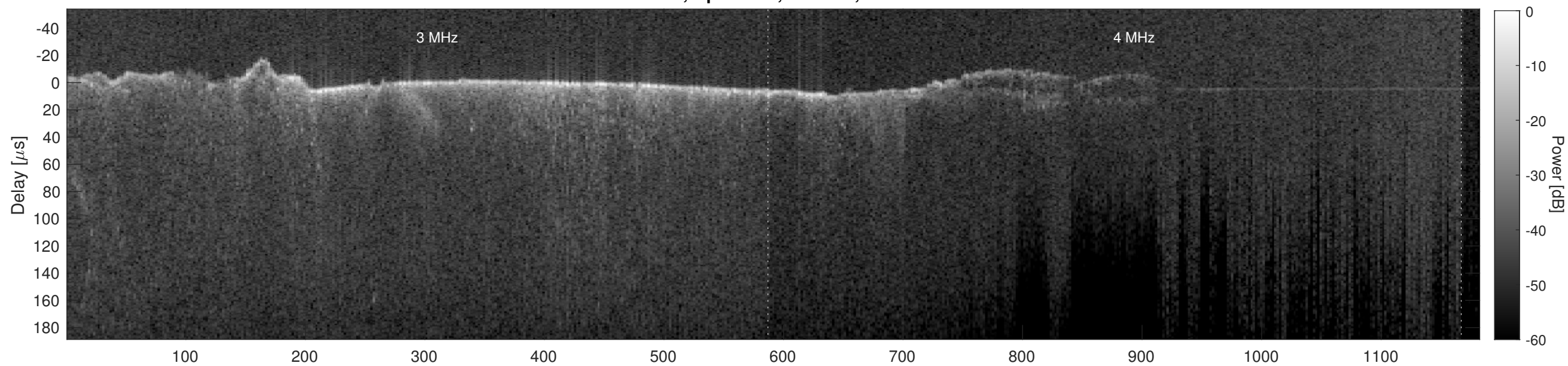
Orbit 3681, Cluttergram
