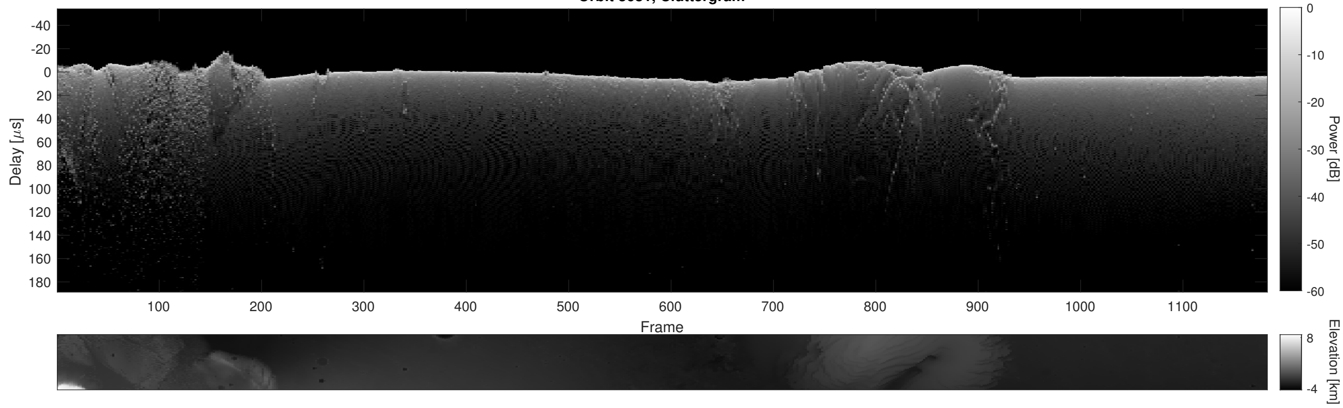
Orbit 3681, Cluttergram
