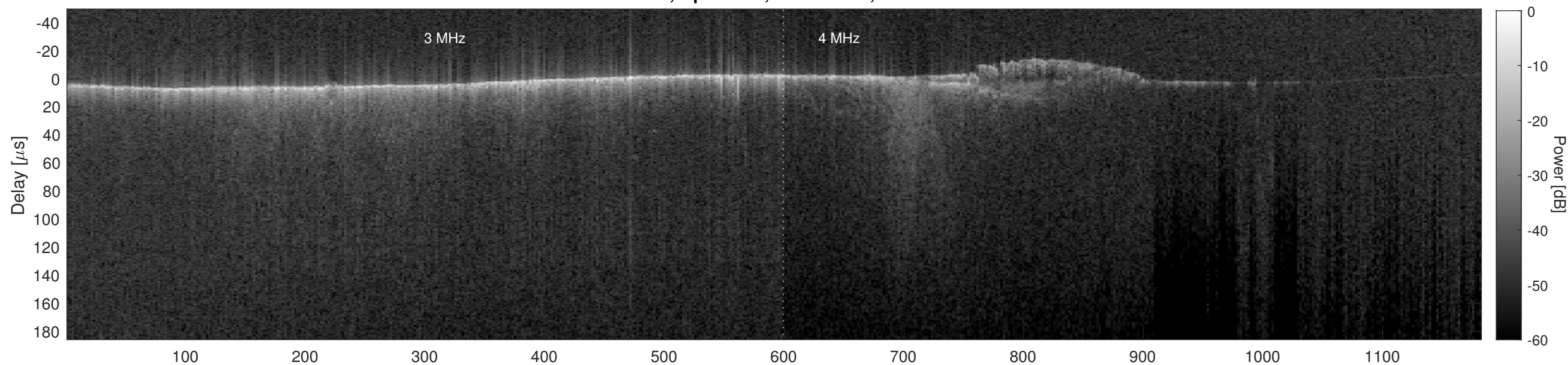
Orbit 3682, Cluttergram
