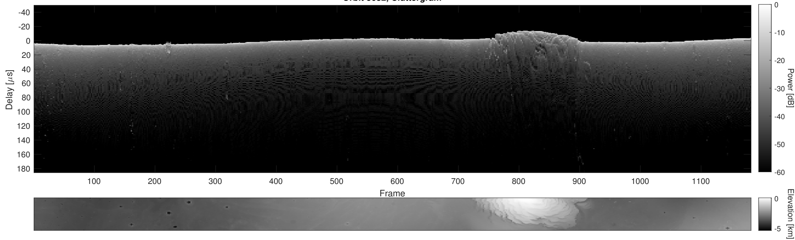
Orbit 3682, Cluttergram
