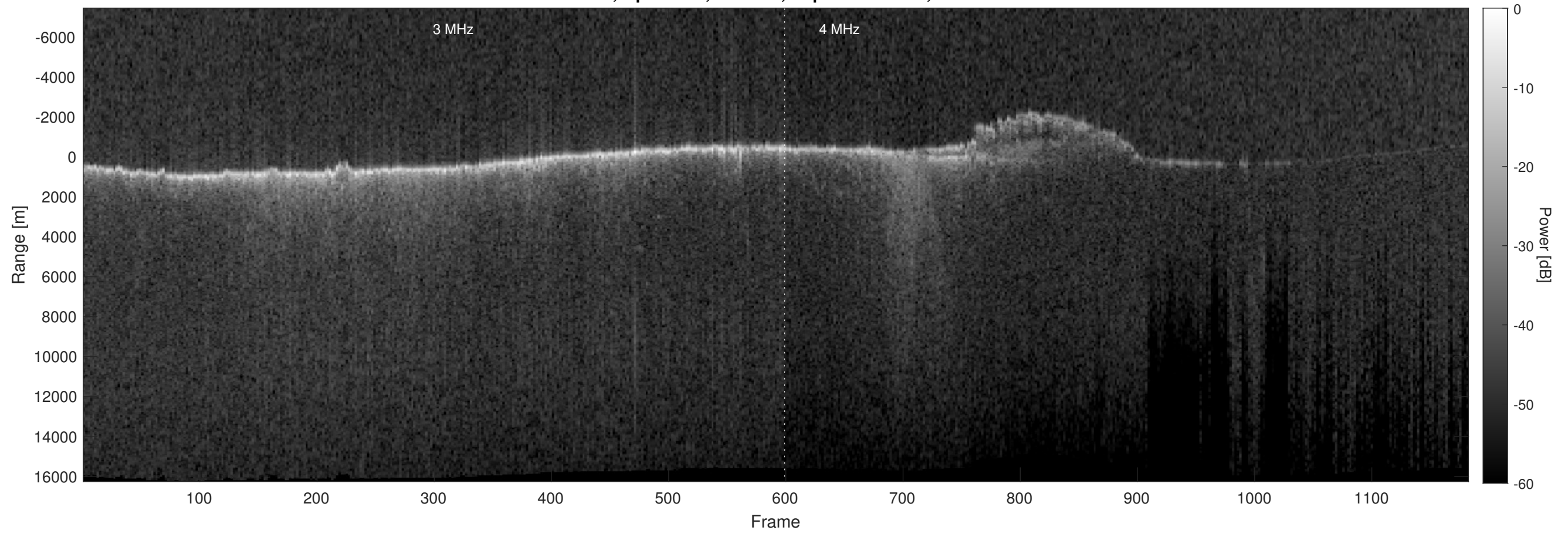
Orbit 3682, Optimized, Window, Depth-Corrected, Channel 2
