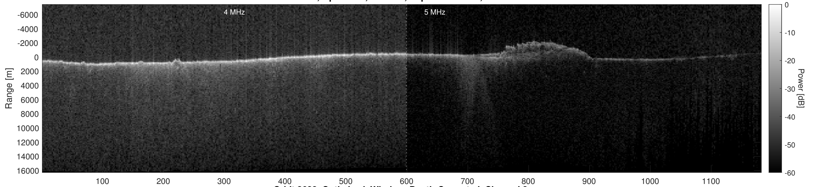
Orbit 3682, Optimized, Window, Depth-Corrected, Channel 2
