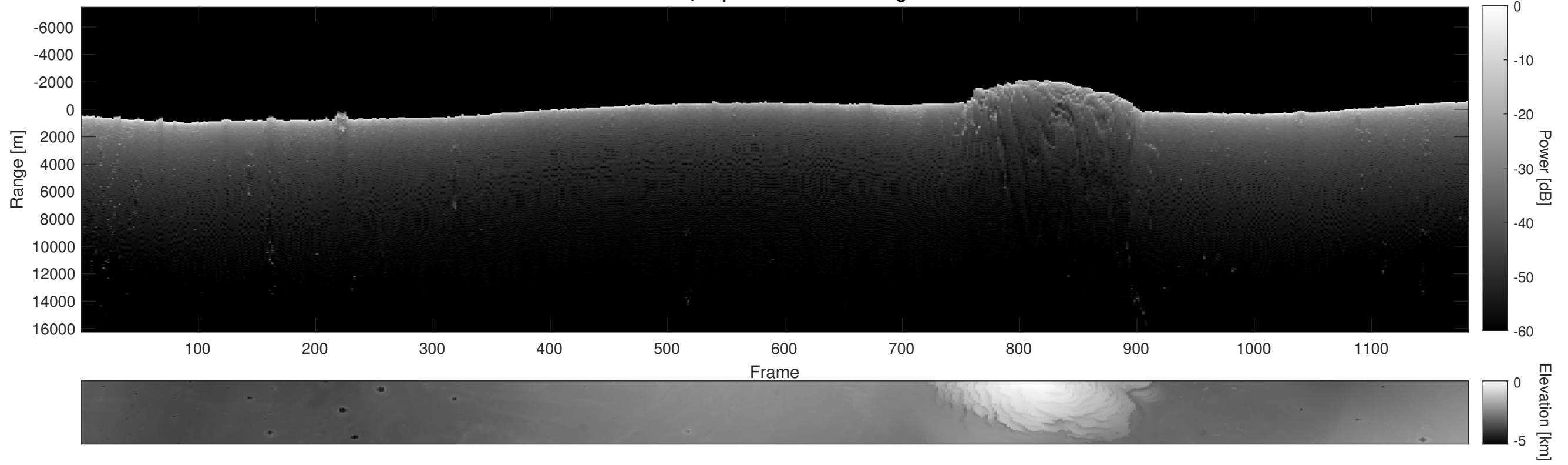
Orbit 3682, Depth-Corrected Cluttergram
