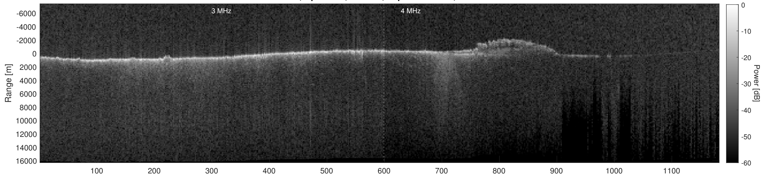
Orbit 3682, Depth-Corrected Cluttergram
