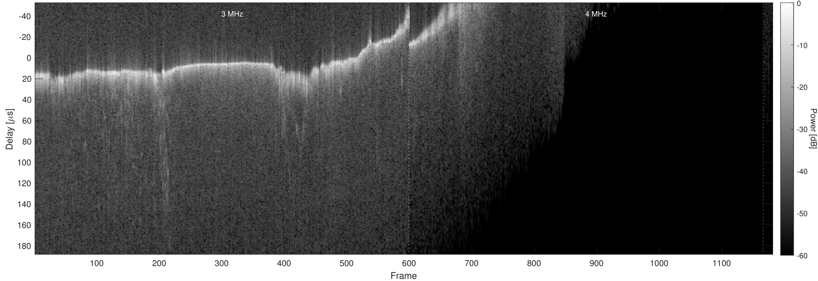
Orbit 3685, Chapman, No Window, Channel 2
