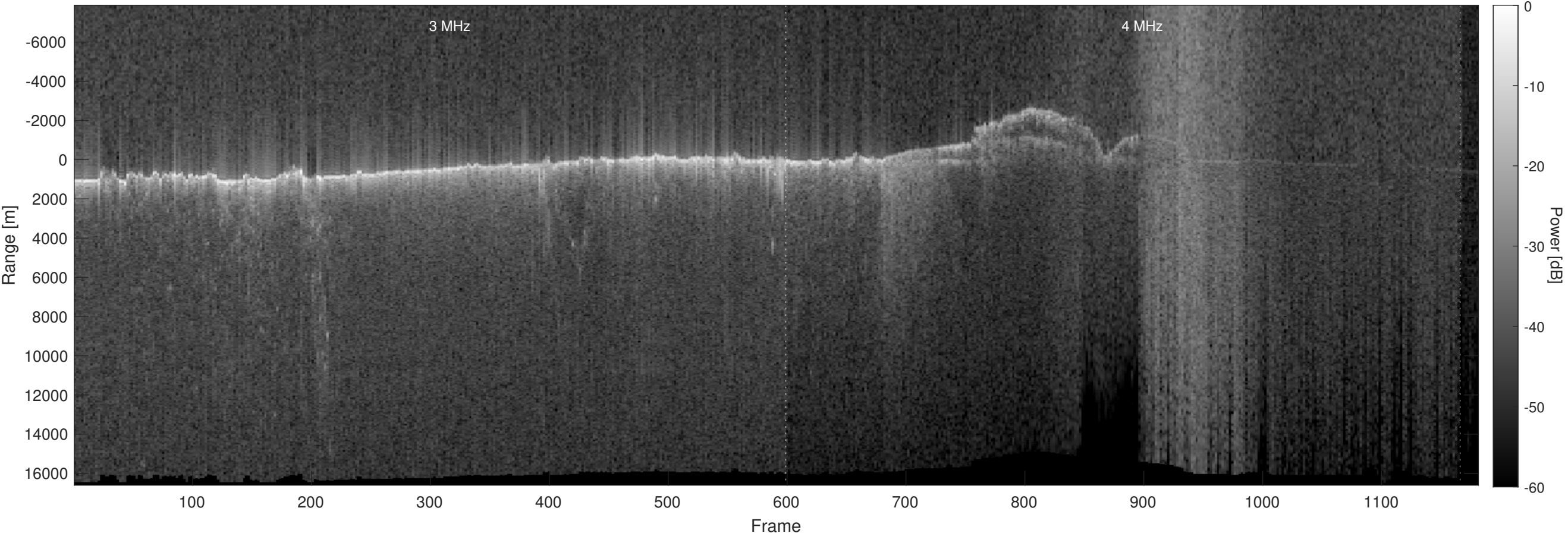
Orbit 3685, Optimized, No Window, Depth-Corrected, Channel 2
