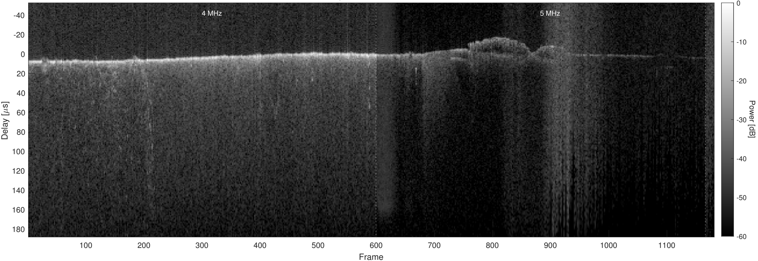
Orbit 3685, Optimized, Window, Channel 2
