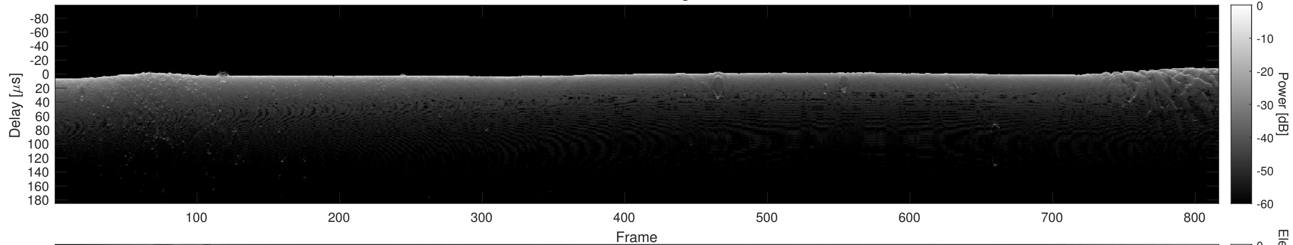
Orbit 3686, Cluttergram
