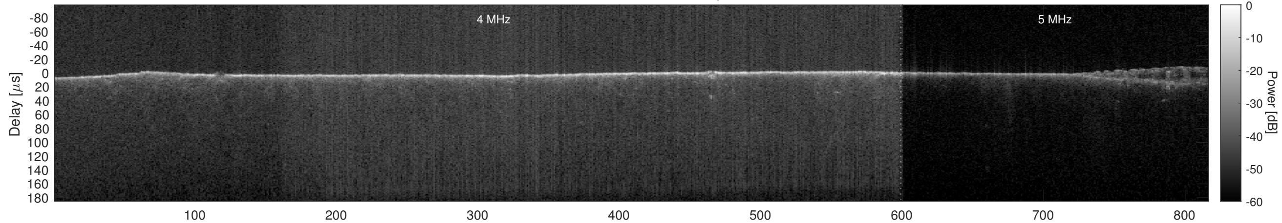
Orbit 3686, Cluttergram
