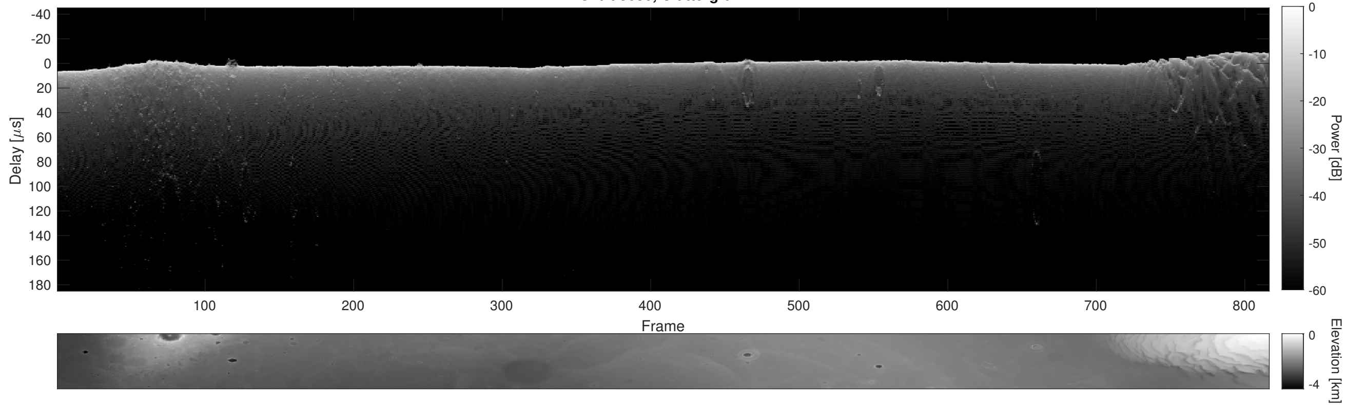
Orbit 3686, Cluttergram
