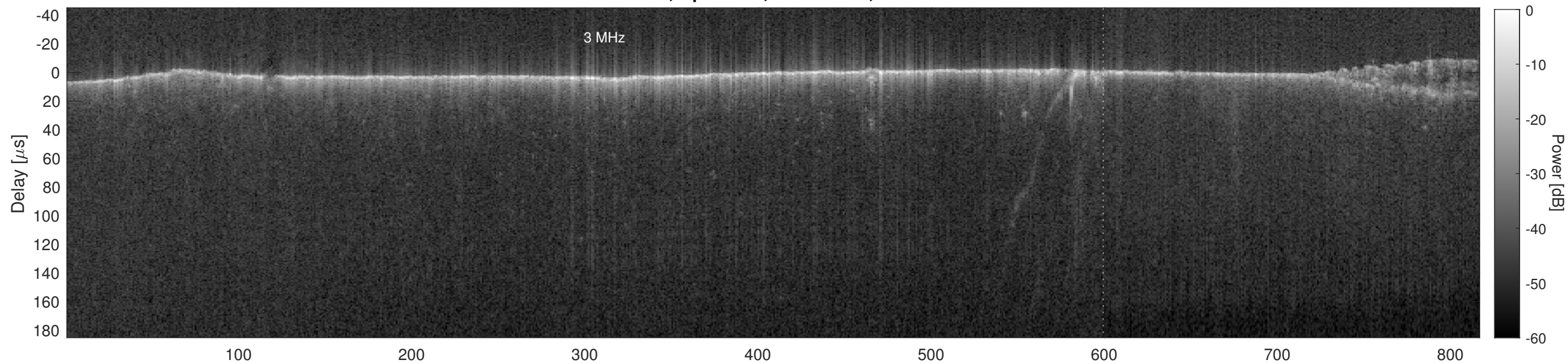
Orbit 3686, Cluttergram
