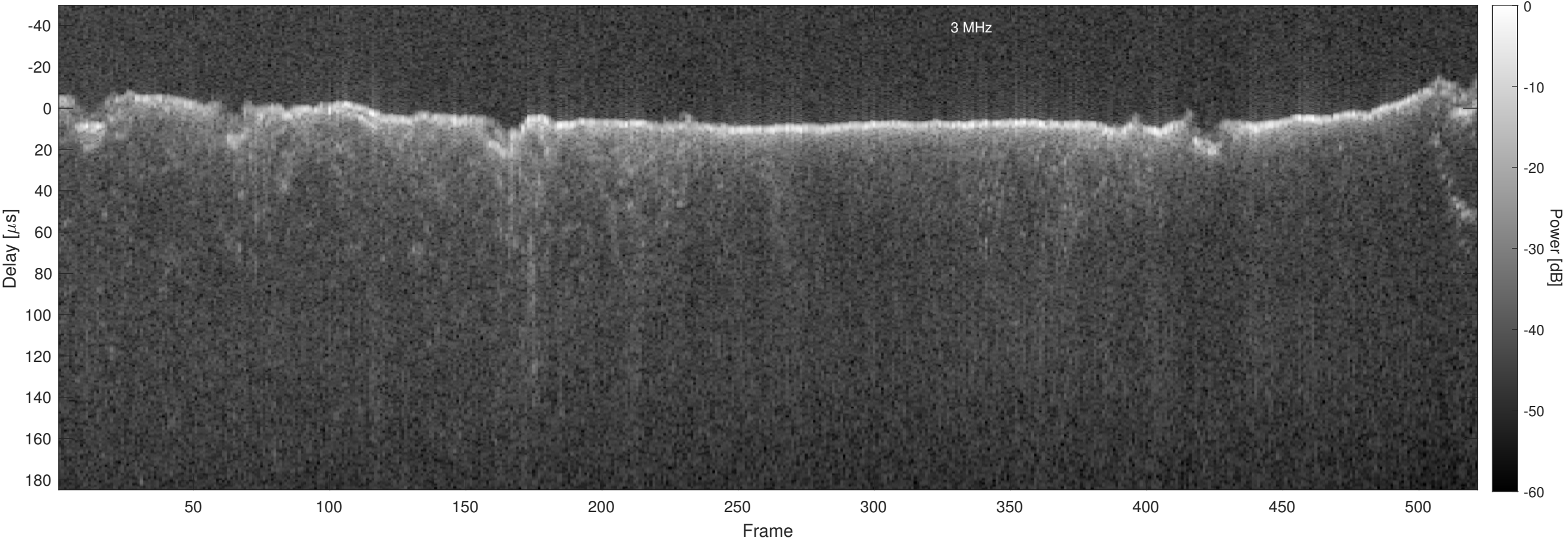
Orbit 3687, Chapman, Window, Channel 2
