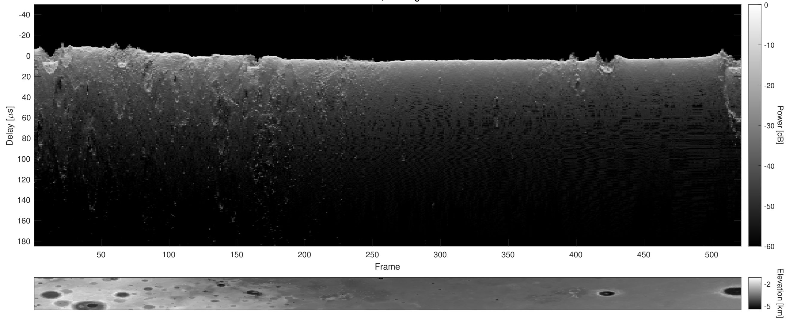
Orbit 3687, Cluttergram
