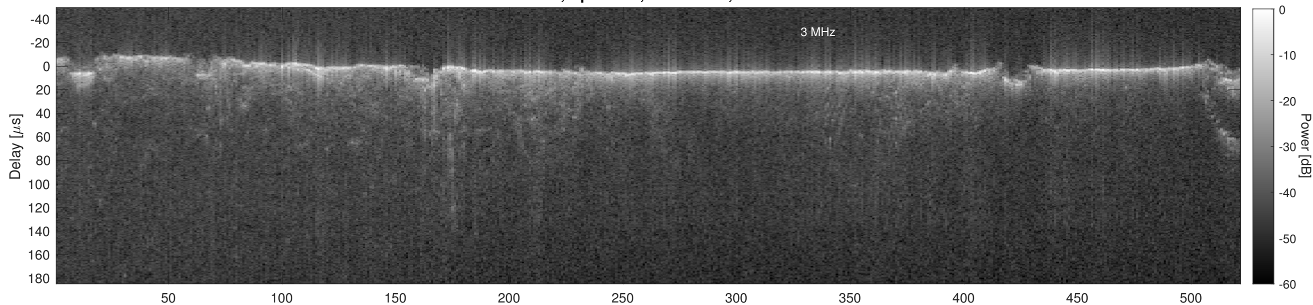
Orbit 3687, Cluttergram
