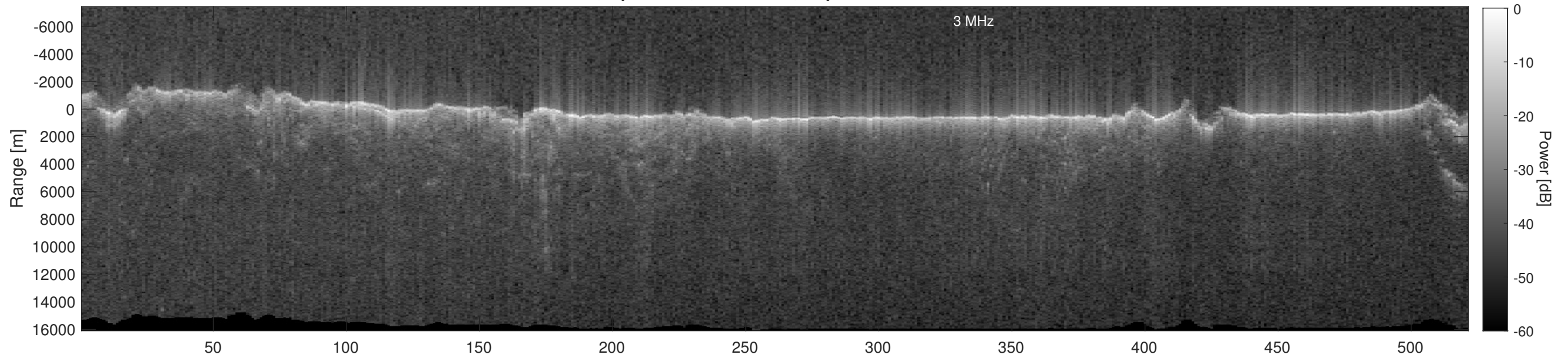
Orbit 3687, Depth-Corrected Cluttergram
