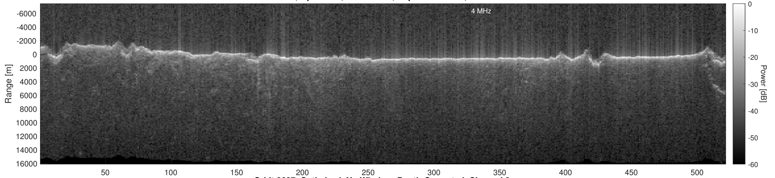
Orbit 3687, Optimized, No Window, Depth-Corrected, Channel 2
