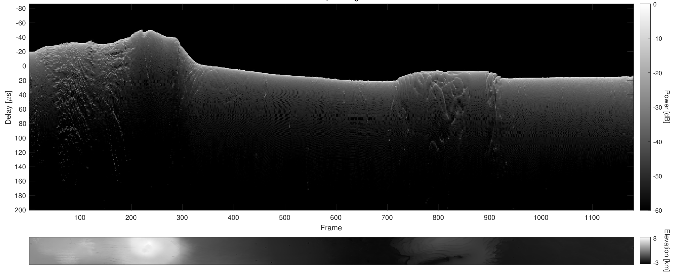
Orbit 3688, Cluttergram
