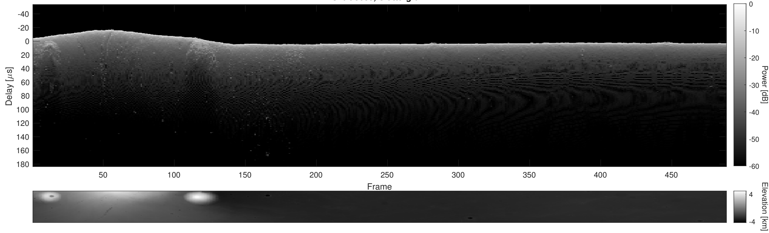
Orbit 3689, Cluttergram
