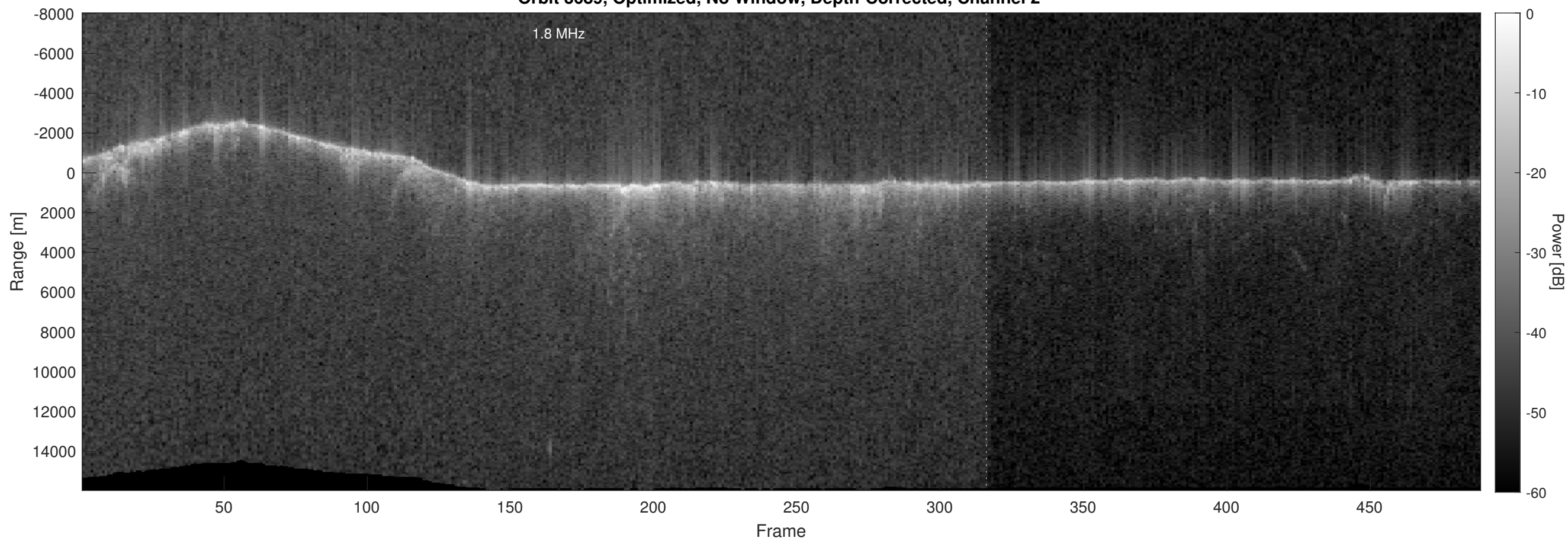
Orbit 3689, Optimized, No Window, Depth-Corrected, Channel 2
