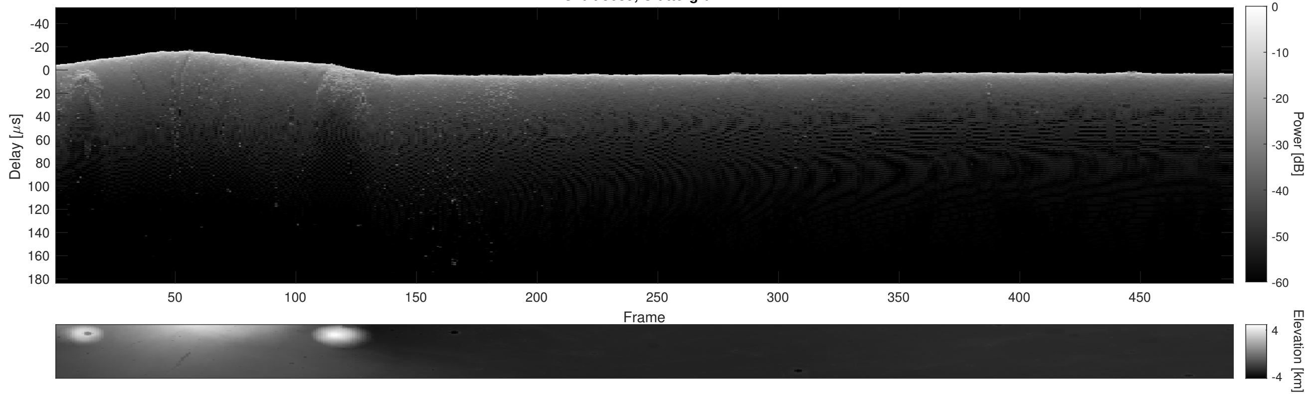
Orbit 3689, Cluttergram
