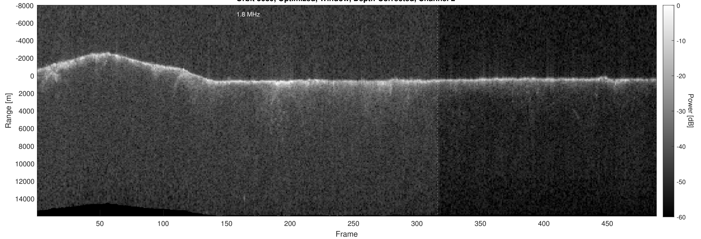
Orbit 3689, Optimized, Window, Depth-Corrected, Channel 2
