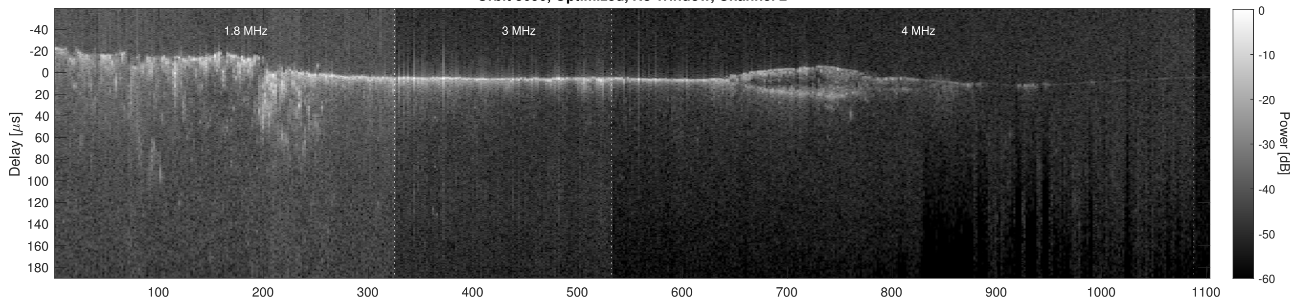
Orbit 3690, Cluttergram
