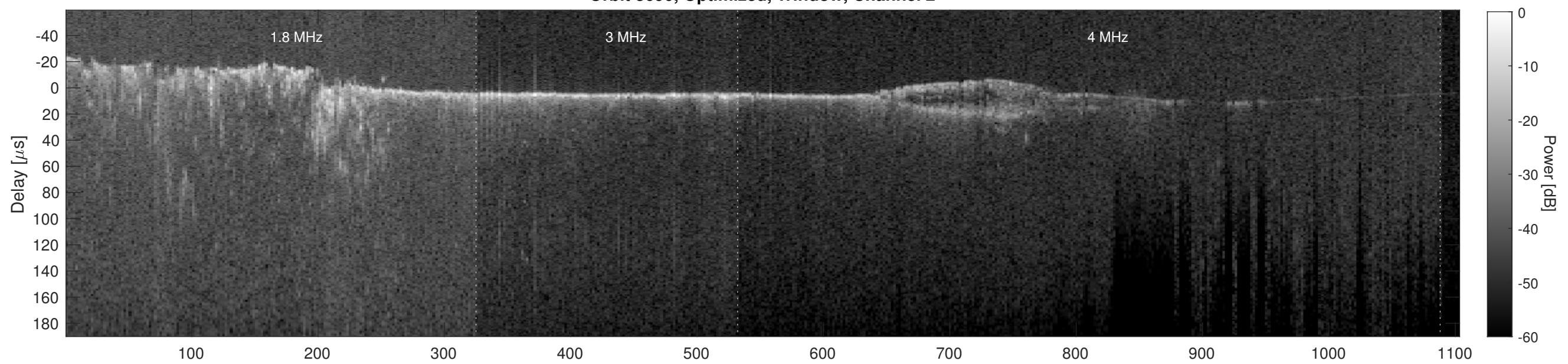
Orbit 3690, Cluttergram
