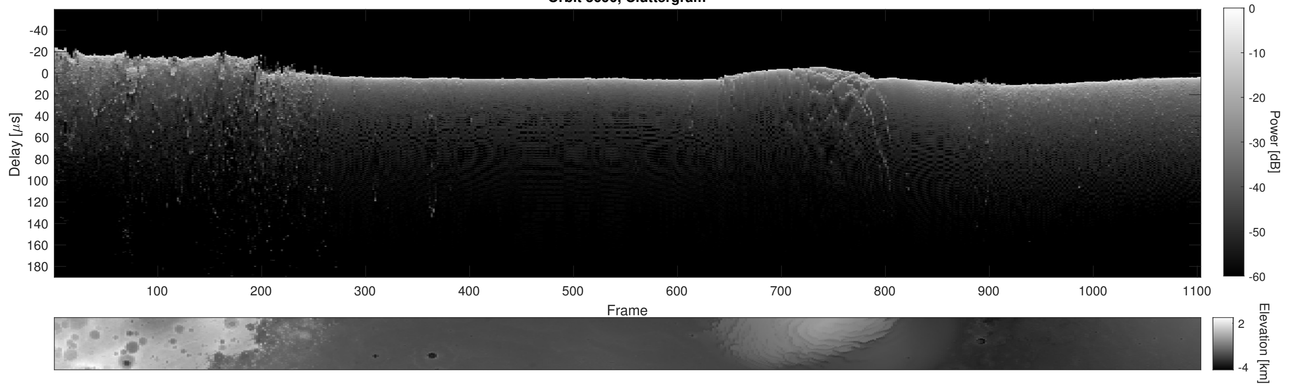
Orbit 3690, Cluttergram
