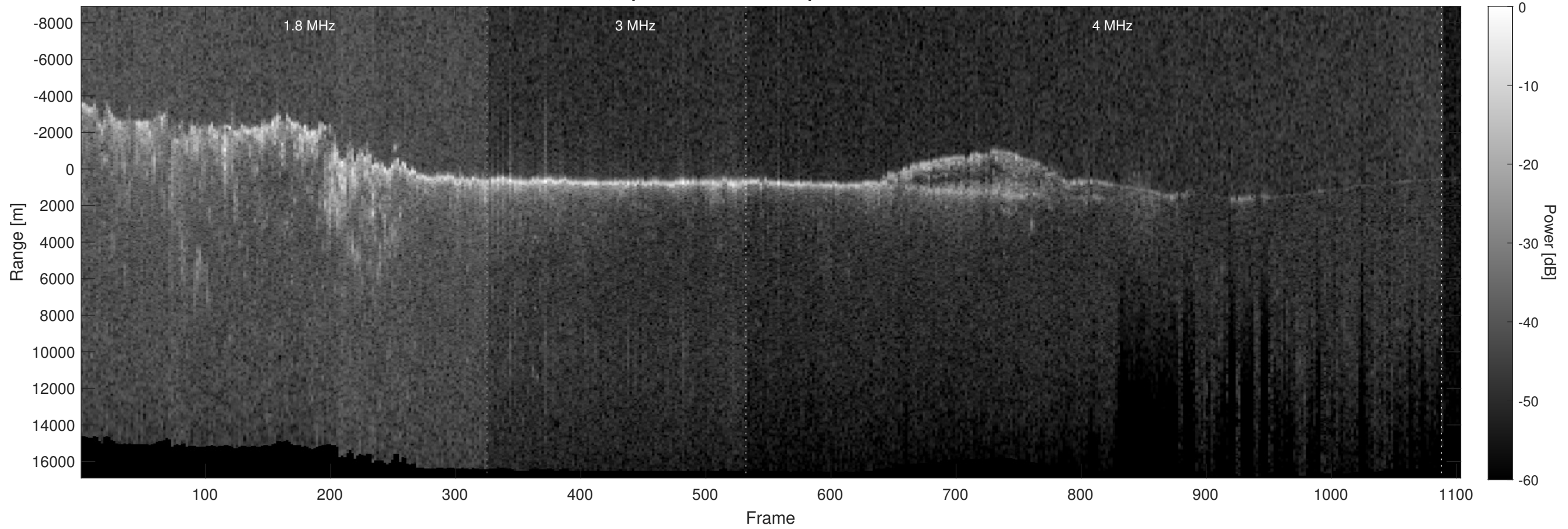
Orbit 3690, Optimized, Window, Depth-Corrected, Channel 2
