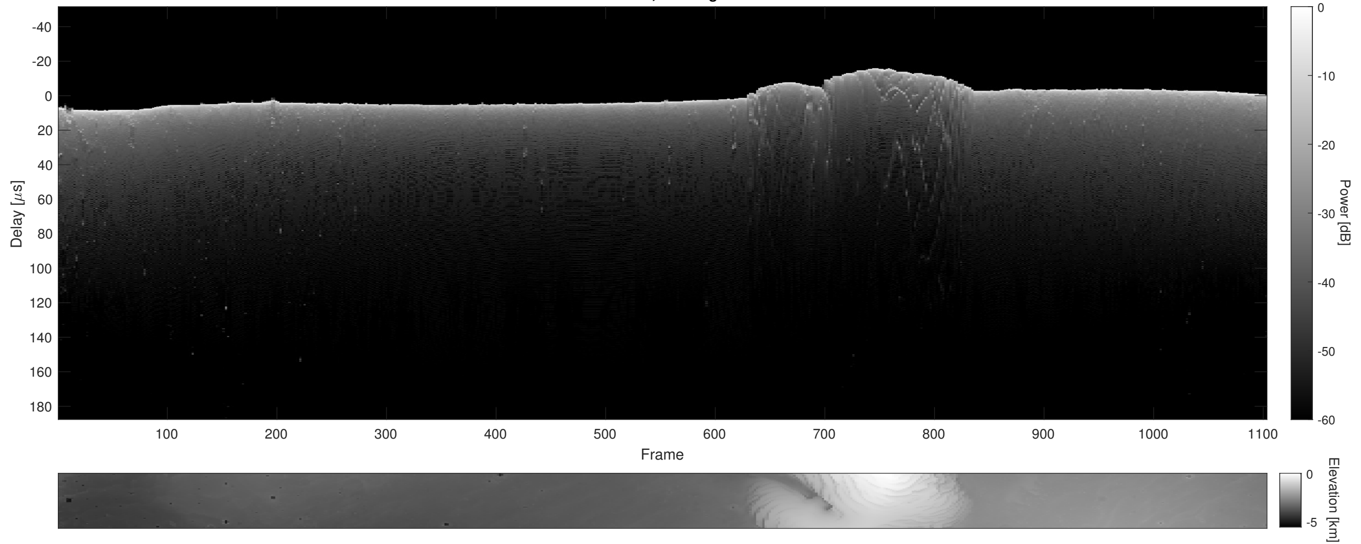
Orbit 3691, Cluttergram
