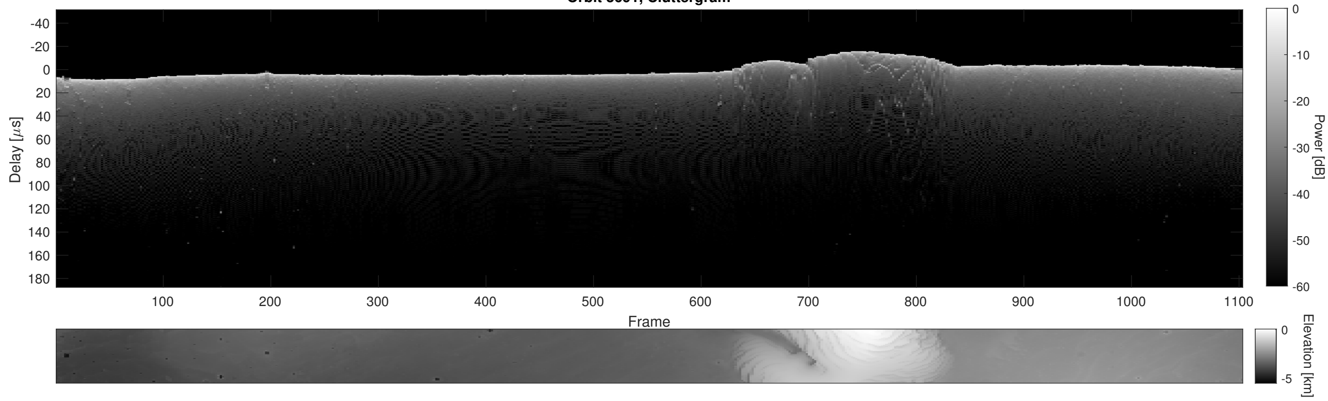
Orbit 3691, Cluttergram
