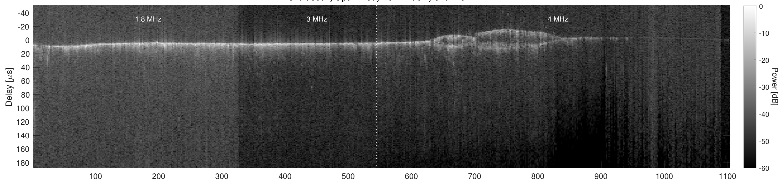
Orbit 3691, Cluttergram
