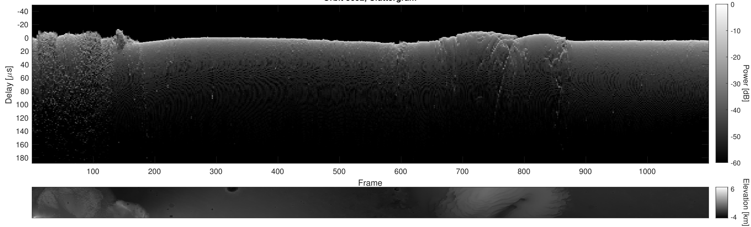
Orbit 3692, Cluttergram
