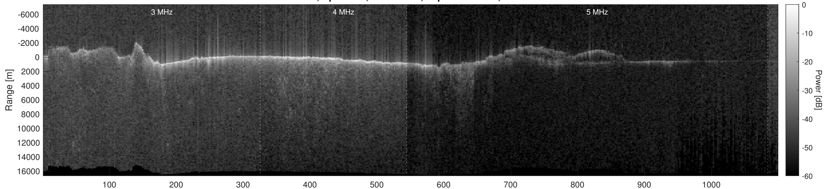
Orbit 3692, Optimized, No Window, Depth-Corrected, Channel 2
