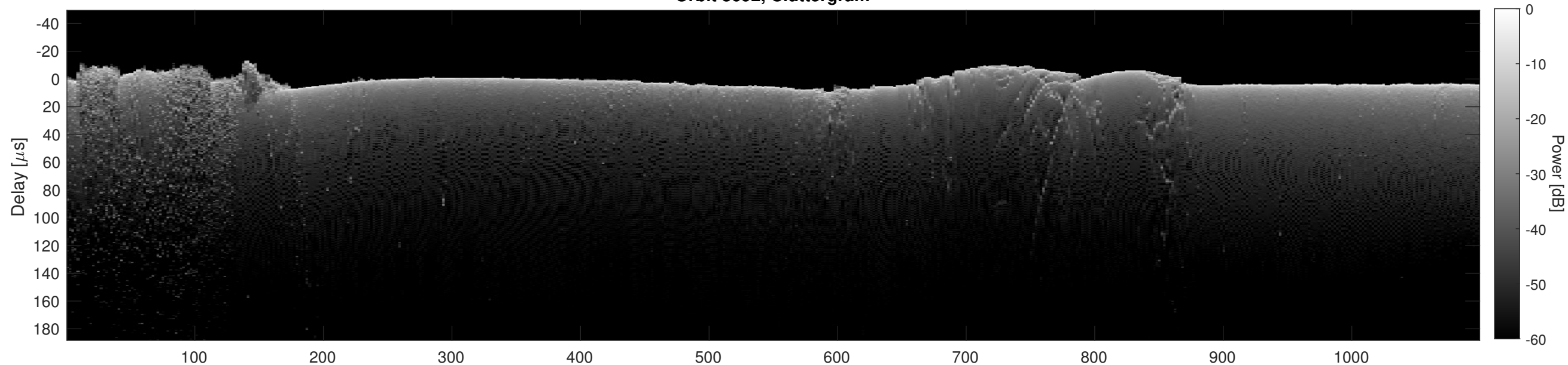
Orbit 3692, Cluttergram
