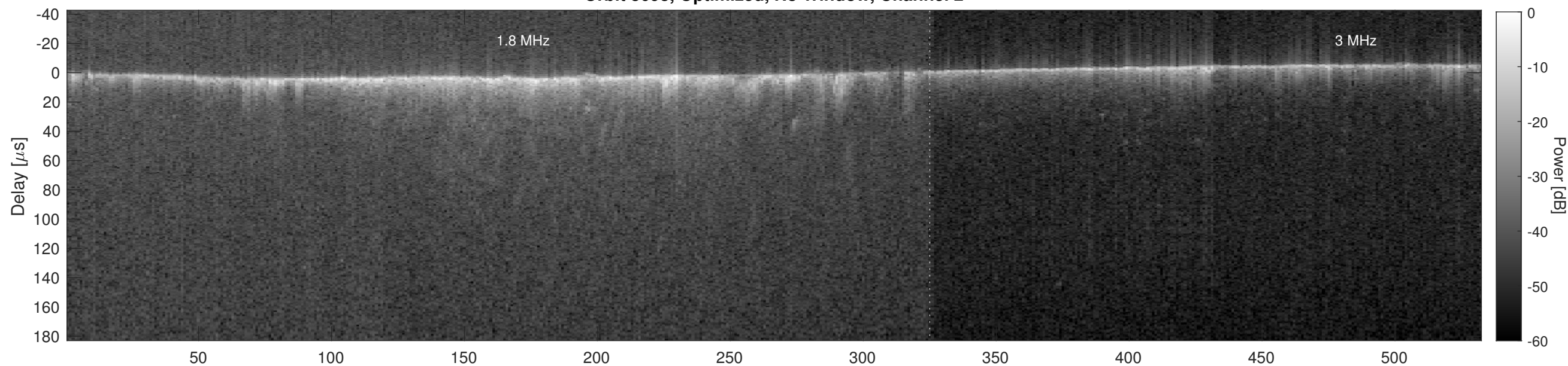
Orbit 3693, Cluttergram
