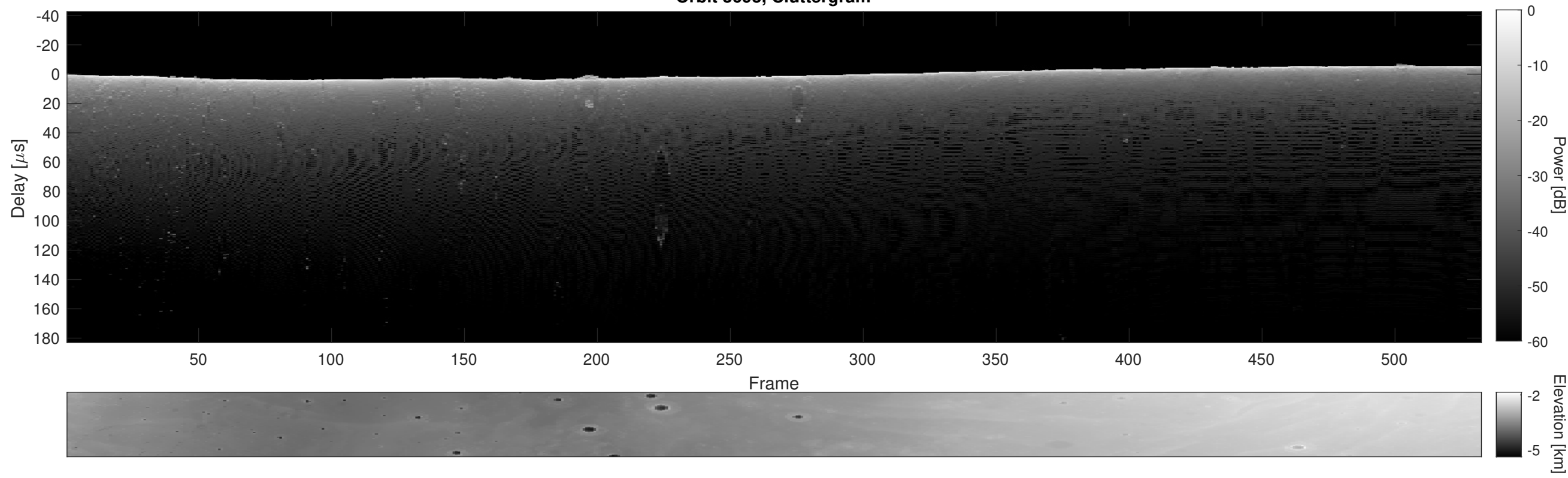
Orbit 3693, Cluttergram
