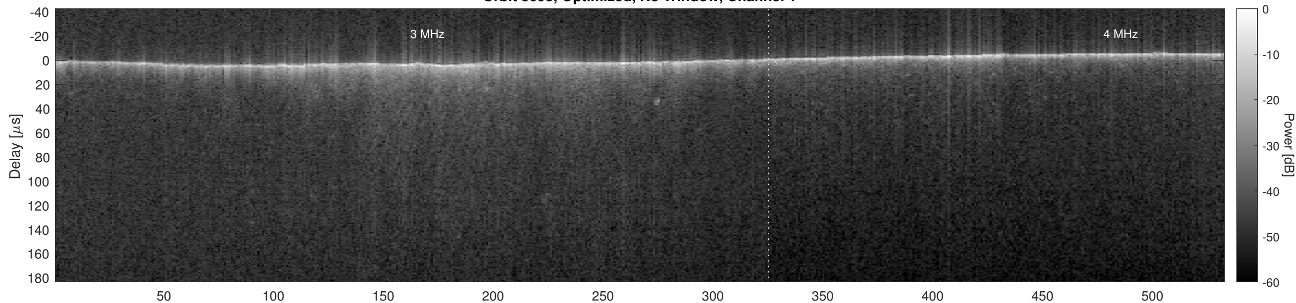
Orbit 3693, Optimized, No Window, Channel 2
