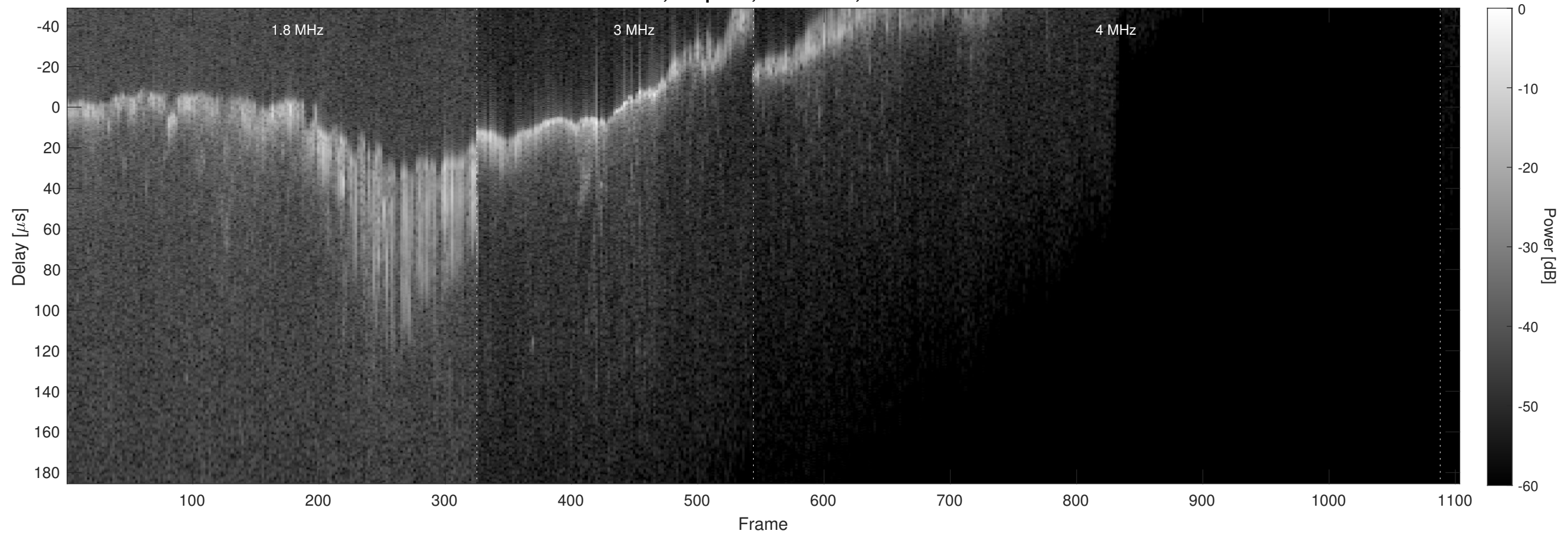
Orbit 3694, Chapman, No Window, Channel 2
