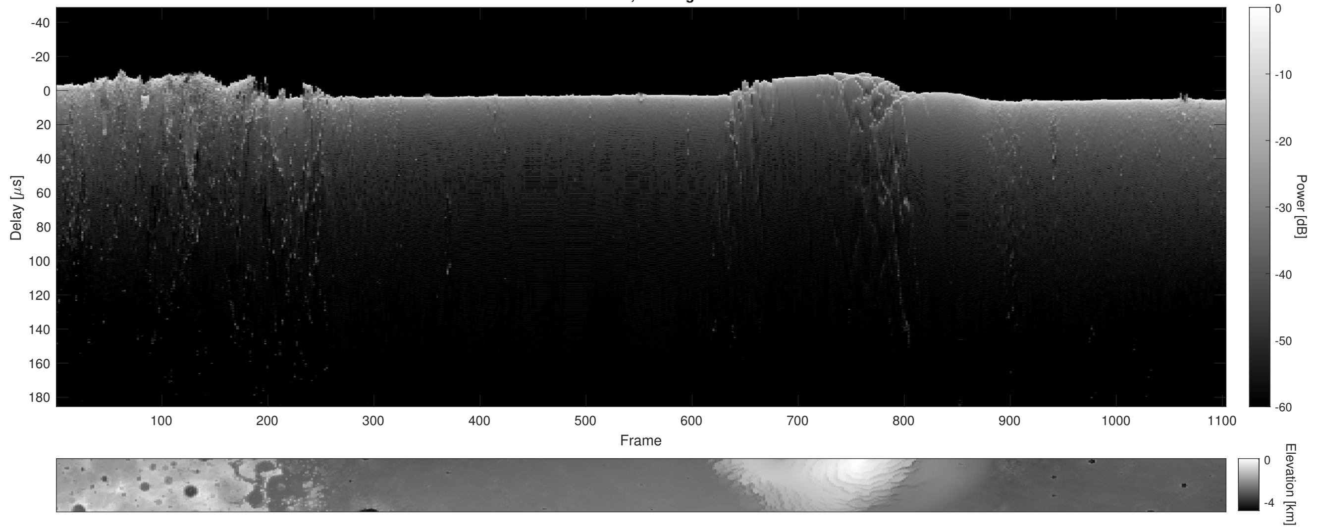
Orbit 3694, Cluttergram
