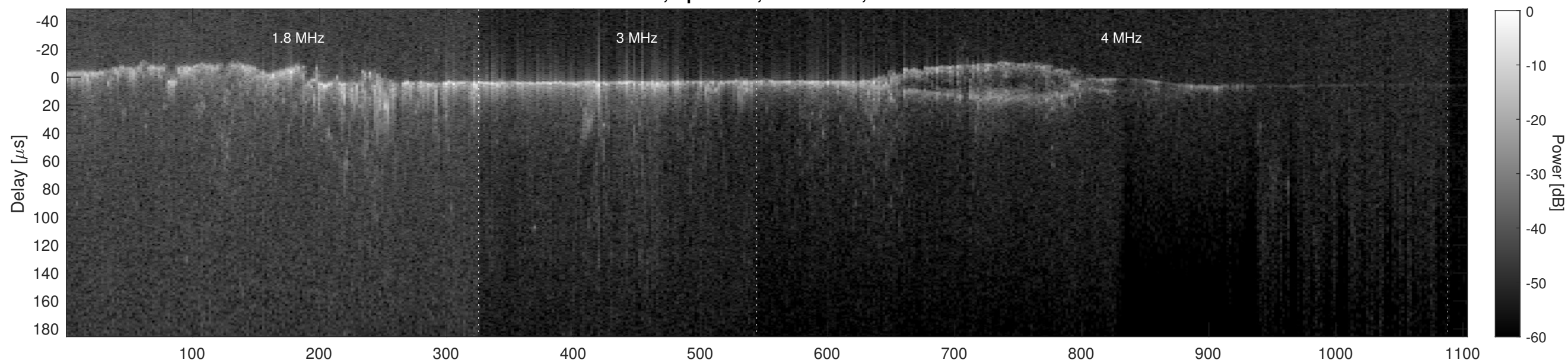
Orbit 3694, Cluttergram
