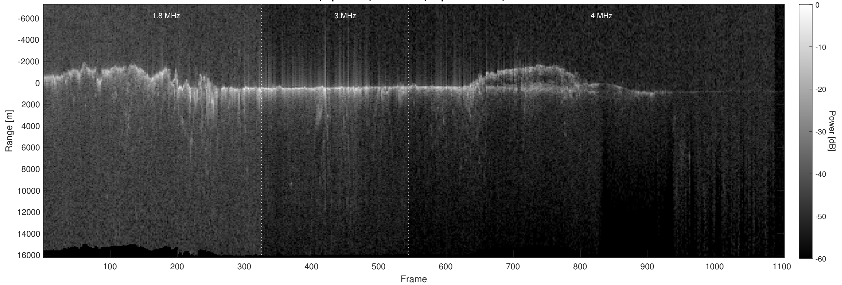
Orbit 3694, Optimized, No Window, Depth-Corrected, Channel 2
