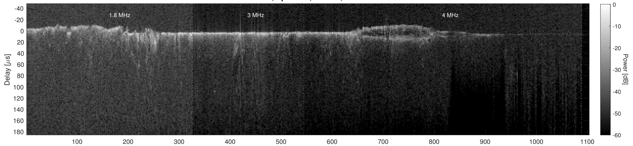
Orbit 3694, Cluttergram
