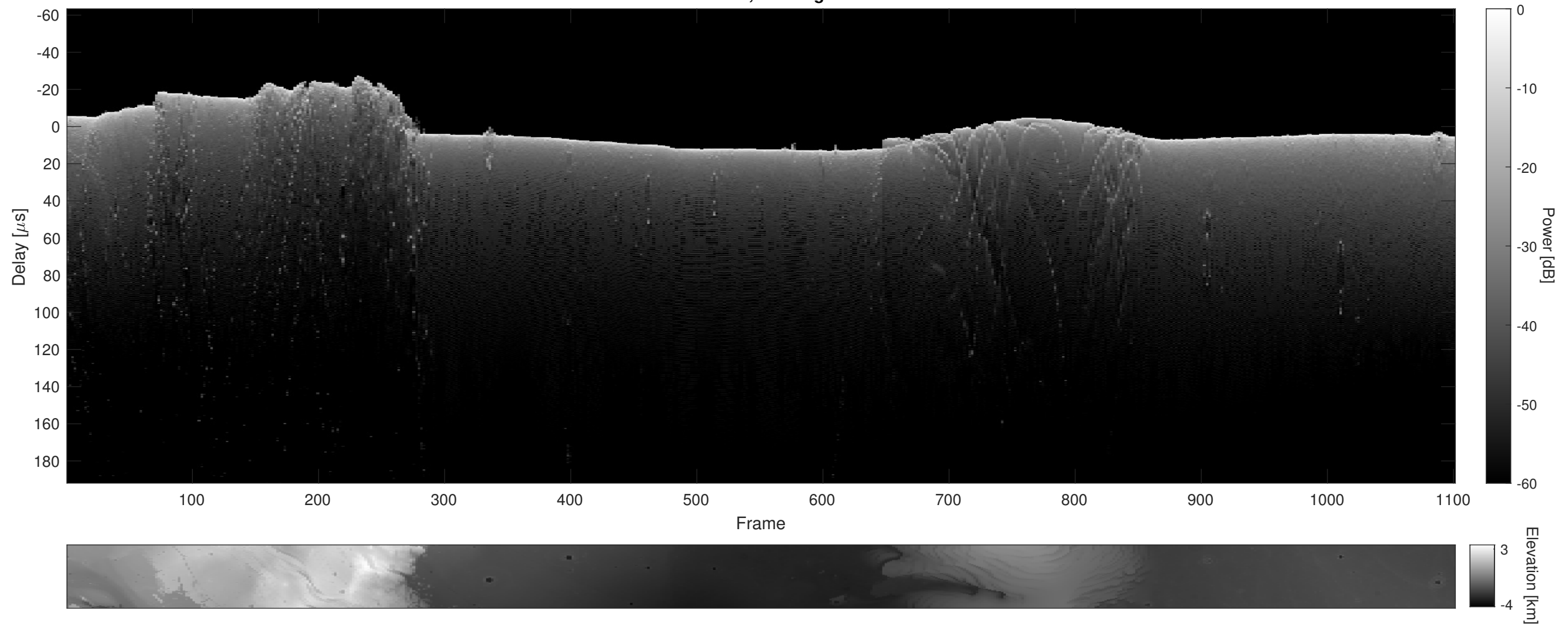
Orbit 3695, Cluttergram
