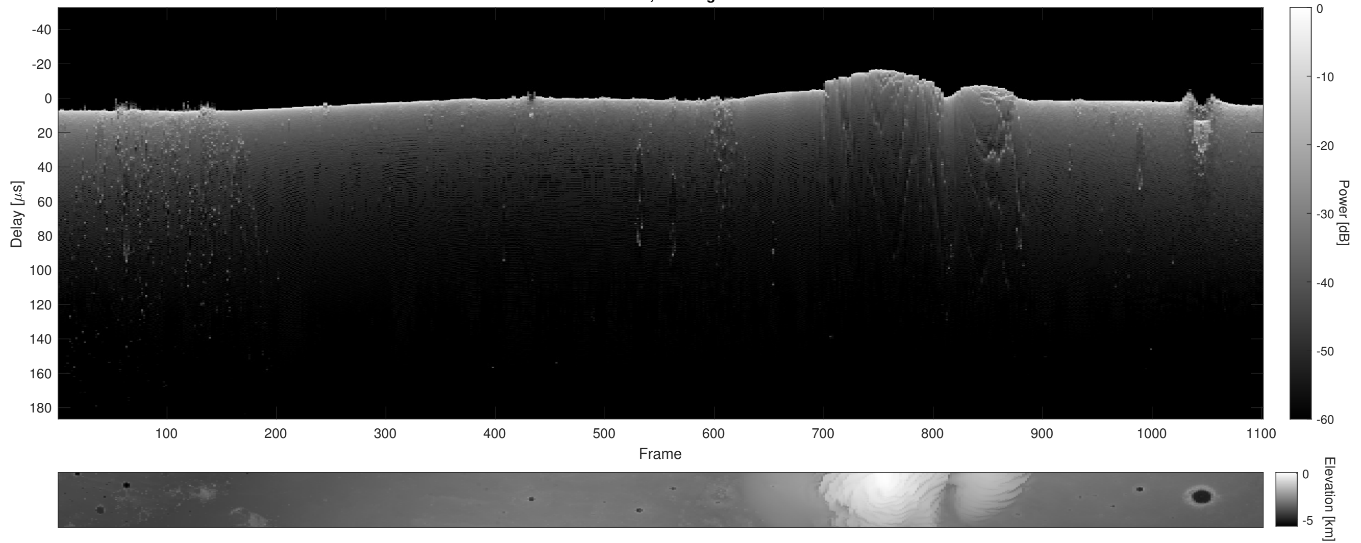
Orbit 3696, Cluttergram
