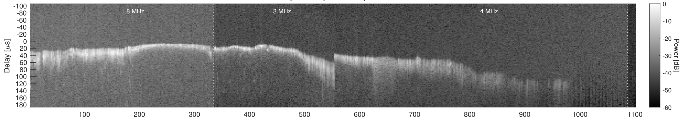
Orbit 3696, Window, Channel 2, Chapman
