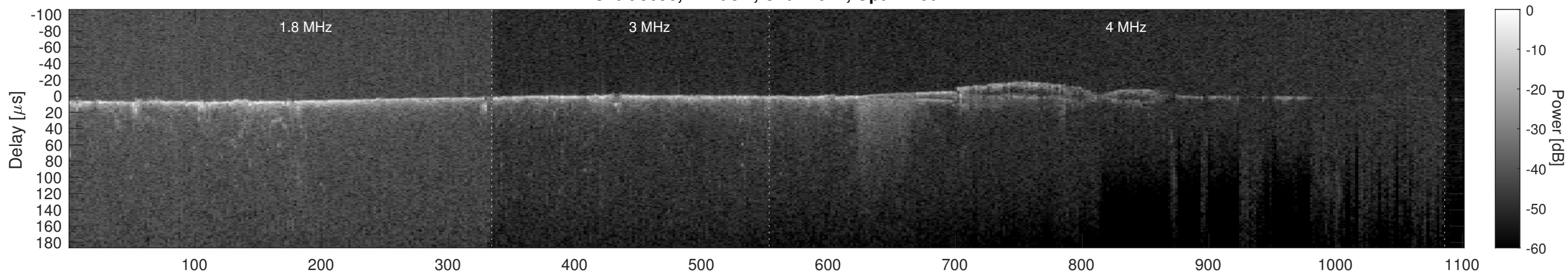
Orbit 3696, Cluttergram
