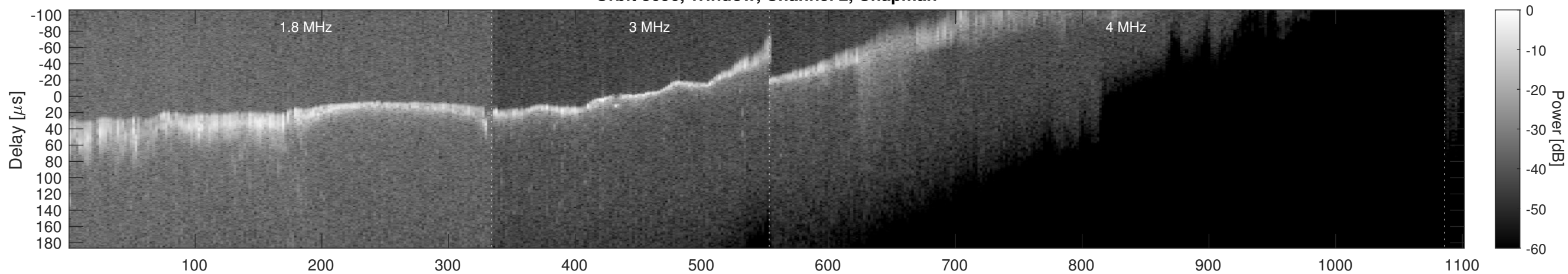
Orbit 3696, Window, Channel 2, Optimized
