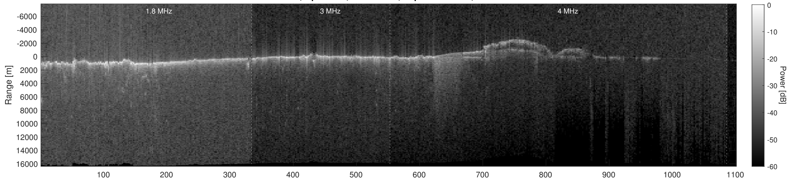
Orbit 3696, Depth-Corrected Cluttergram
