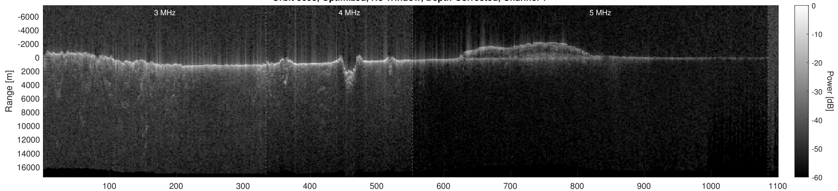
Orbit 3698, Optimized, No Window, Depth-Corrected, Channel 2
